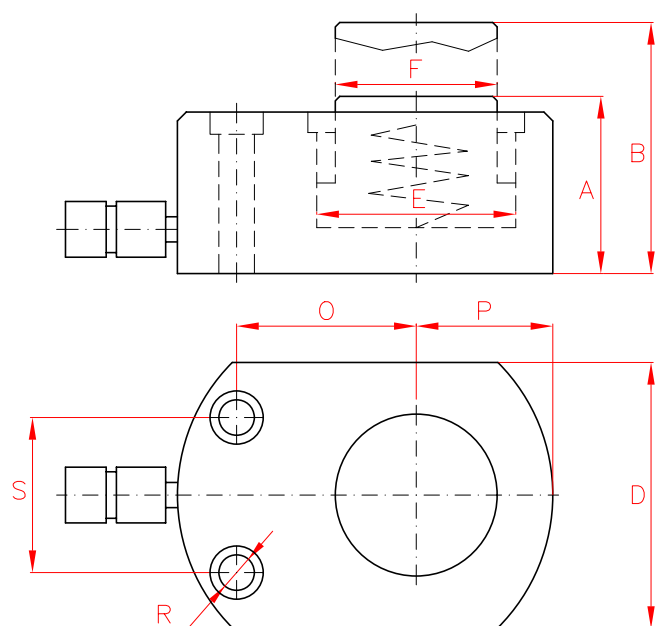
SMX spring return
